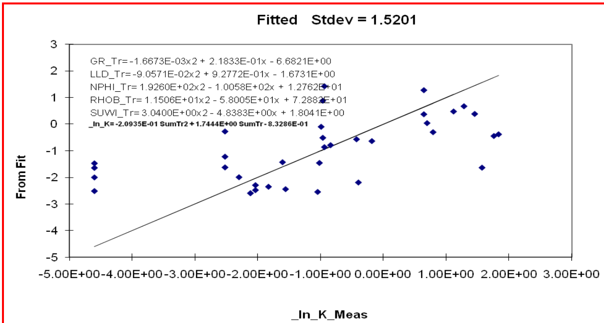
Figure-8: Fitted Standard Deviation
