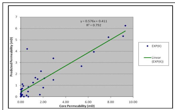
Figure-12: Linear trendline, between core k and predicted k data
