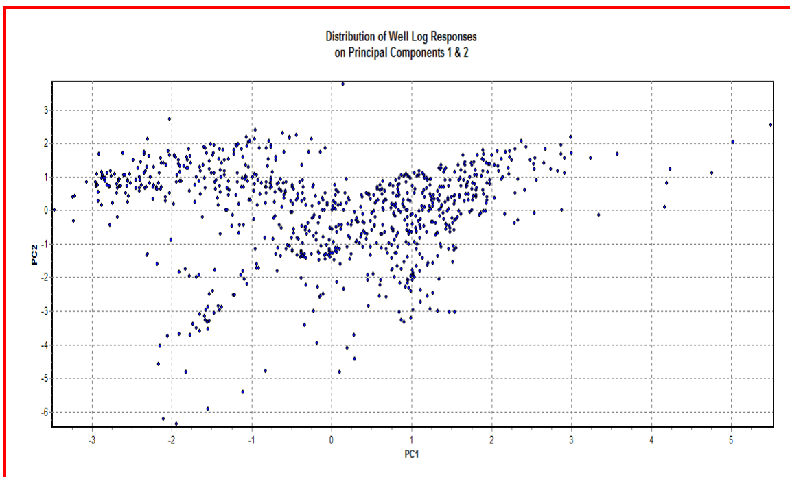
Figure-4: Scatter plot of the sample data set from Wells A, B and C
