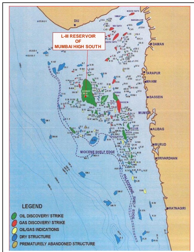
Figure-1: Location Map Bombay Offshore Basin
