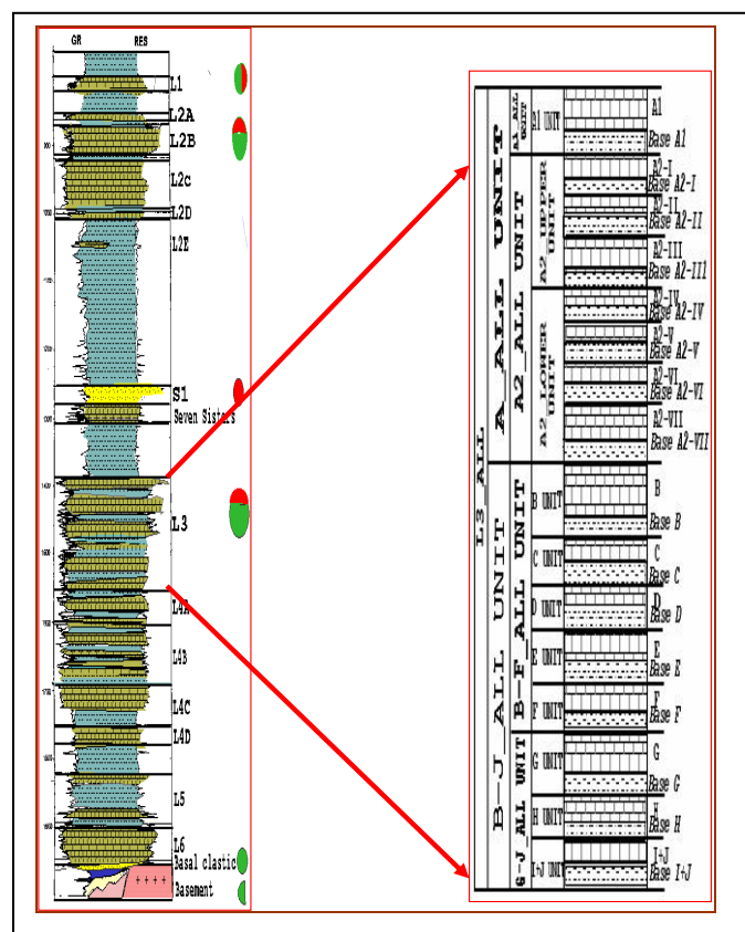
Figure-2: General Stratigraphy Mumbai High Field
