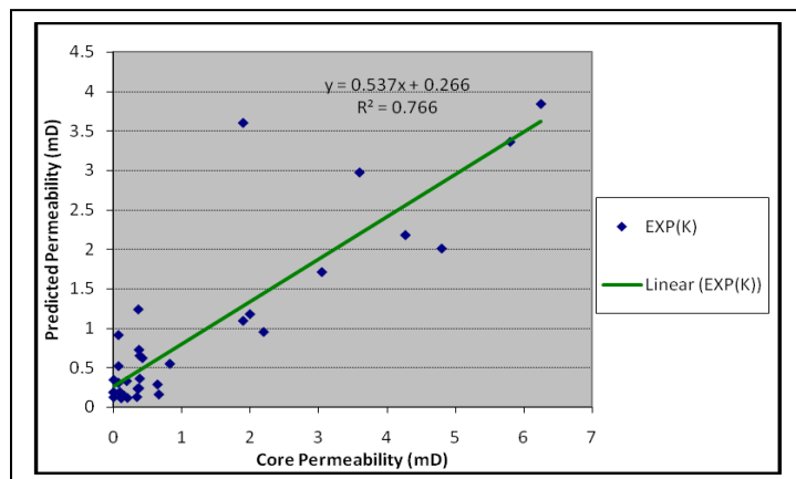
Figure-11: Linear trendline, between the core and predicted k data
