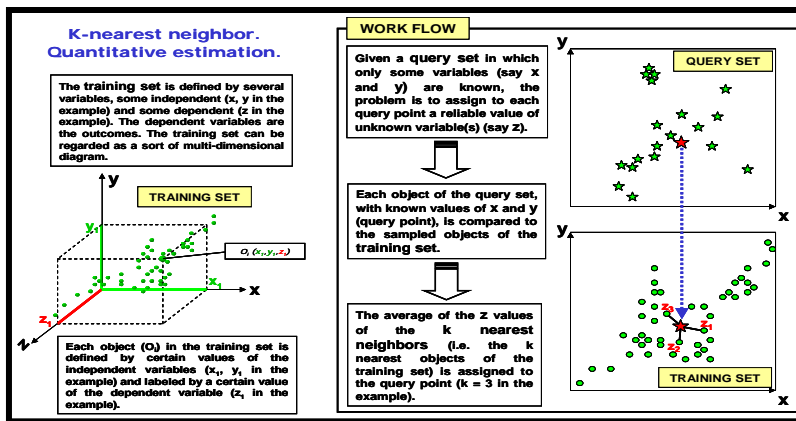
Fig.2 Key Nearest Neighbour methodology
