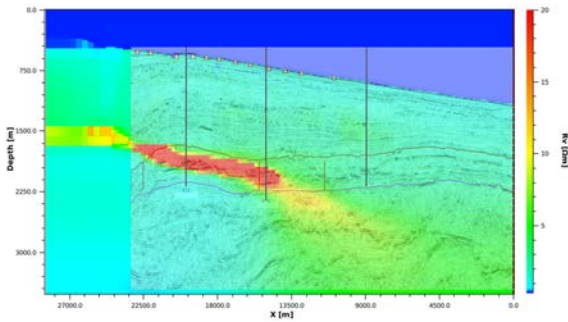
Figure 6: 2.5D unconstrained inversion result overlain with seismic for line 01 in offshore KG basin, India
