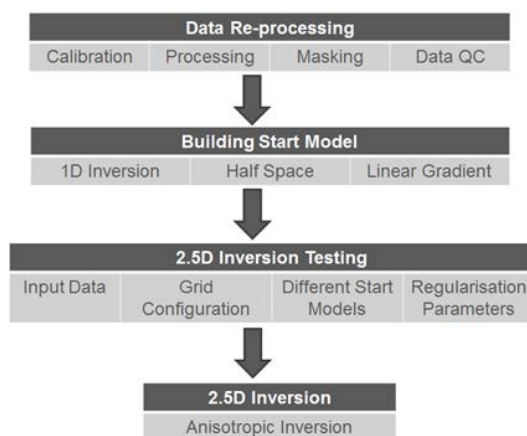
Figure 2: Processing & 2.5D Inversion Workflow
