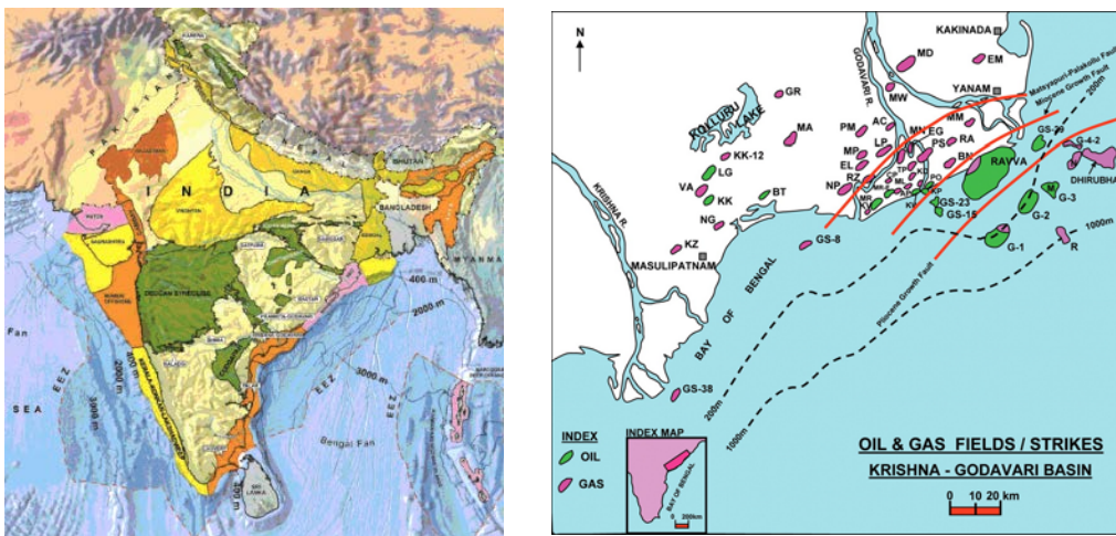
Figure 1: Location Map of Krishna-Godavari basin
