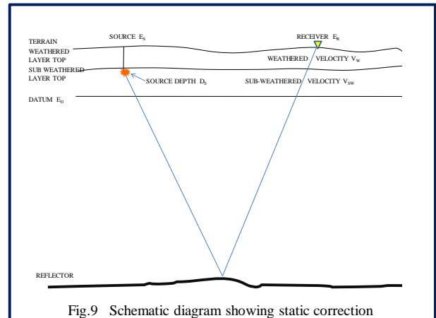
Fig.9 Schematic diagram showing static correction
