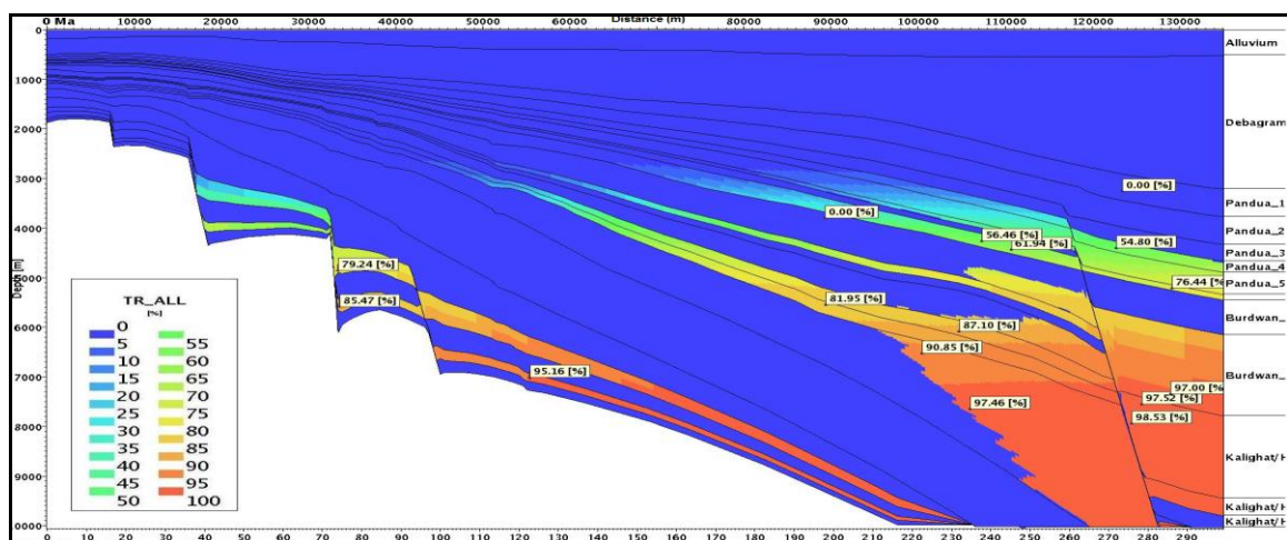
Figure-7: Modeled Transformation Ratio (% TR) at 0 Ma (present day)
