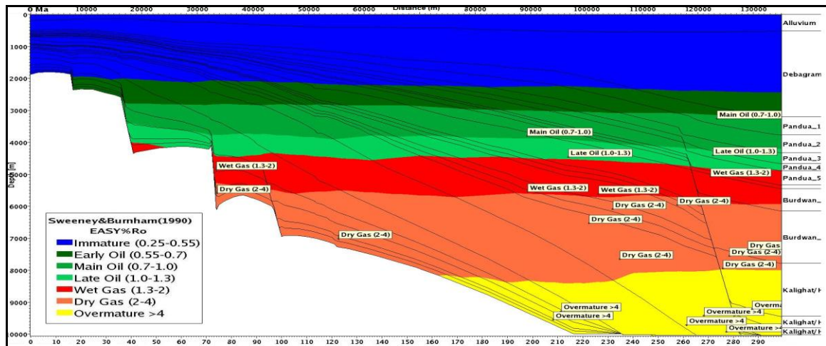
Figure-6: Modeled Maturity (% VRo) at 0 Ma (present day)
