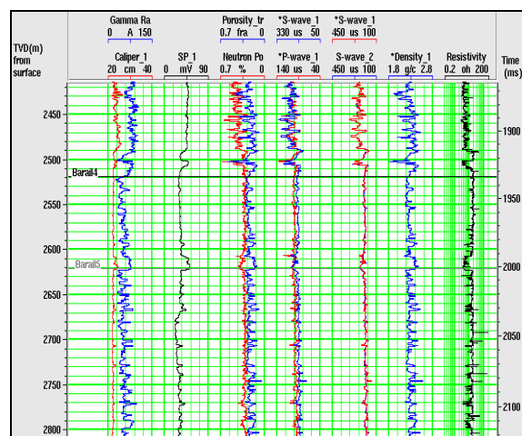
Fig. 2C : Details of logs in the Barail 4 & 5 intervals Well A
