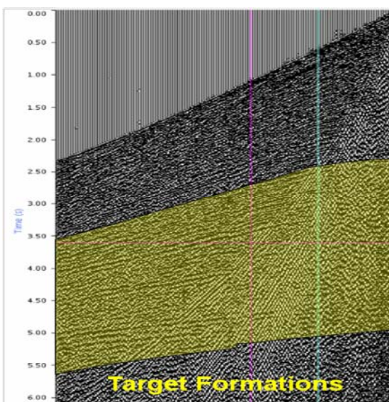
Figure- 6C: PSV wave component
