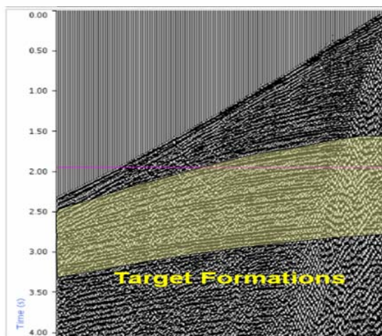
Figure- 6A: P wave component
