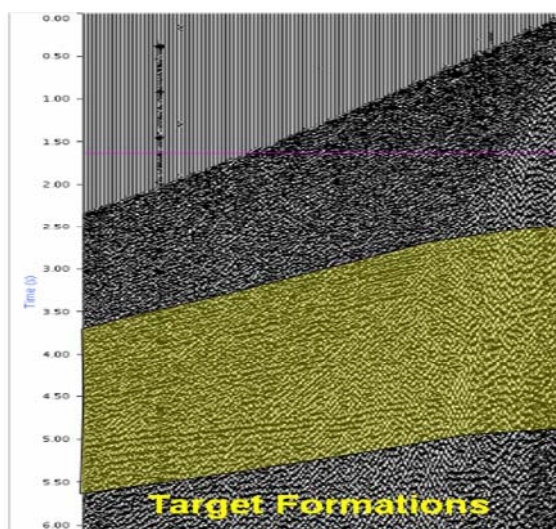
Figure- 6B: PSH wave component
