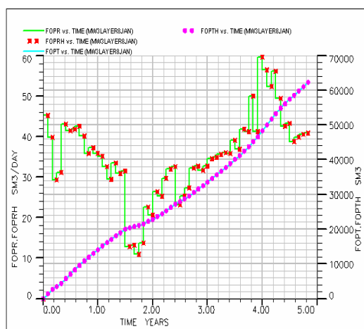
Fig. 7 History Match of Oil Production Block of MW#16, BCS-III Sand
