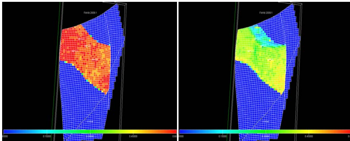
Fig. 9 Oil Saturation Map, Initial and At the End of History
