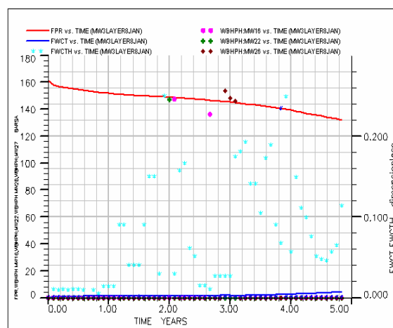
Fig. 8 History Match of Pressures Block of MW#16, BCS-III Sand
