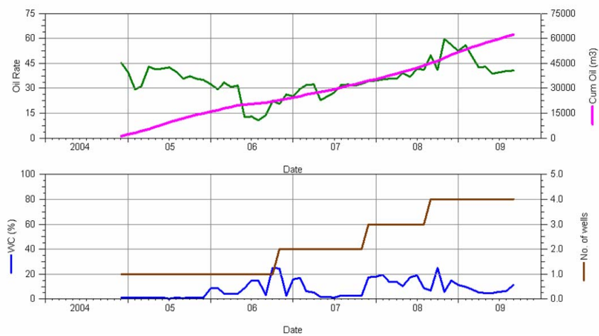
Fig. 4 Performance History of Block of MW#16
