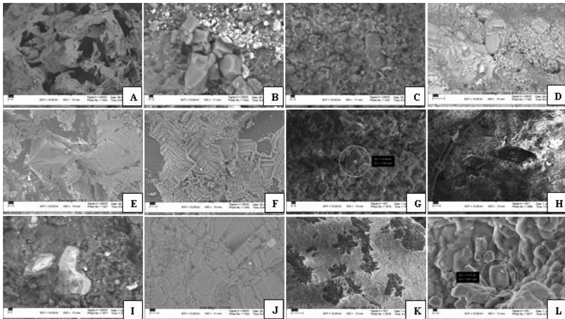
Fig.3- SEM photographs of some caprock samples: A)-Network anhydrite with dissolved halite pores (well 25, 3288m); B)-Euhedral anhydrite crystals (well19, 3389m); C)- Shale (well 4, 3366m); D)-Deformed anhydrite (well 40, 3395m); E & F)-Hopper and chevron textures in halite (well 4, 3449m); G)- Euhedral anhydrite (well 30, 3306); H)-Automorph calcite in anhydrite matrix (well 22, 3355m); I)- Barite crystals (well 30, 3314m); J)- Compact anhydrite (well 30, 3366m); K)-Star shaped anhydrite (well40, 3376m); and L)- Rhombohedron anhydrite (well 25, 3289m).
