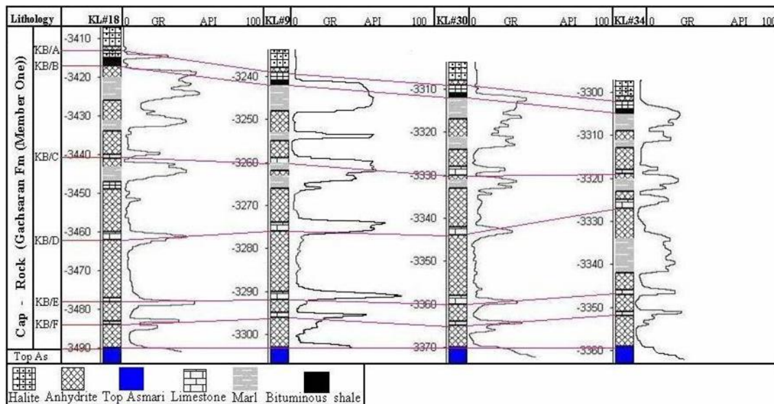
Fig.1- General stratigraphic column correlation and Gamma Ray Log. Depth is in per meter.
