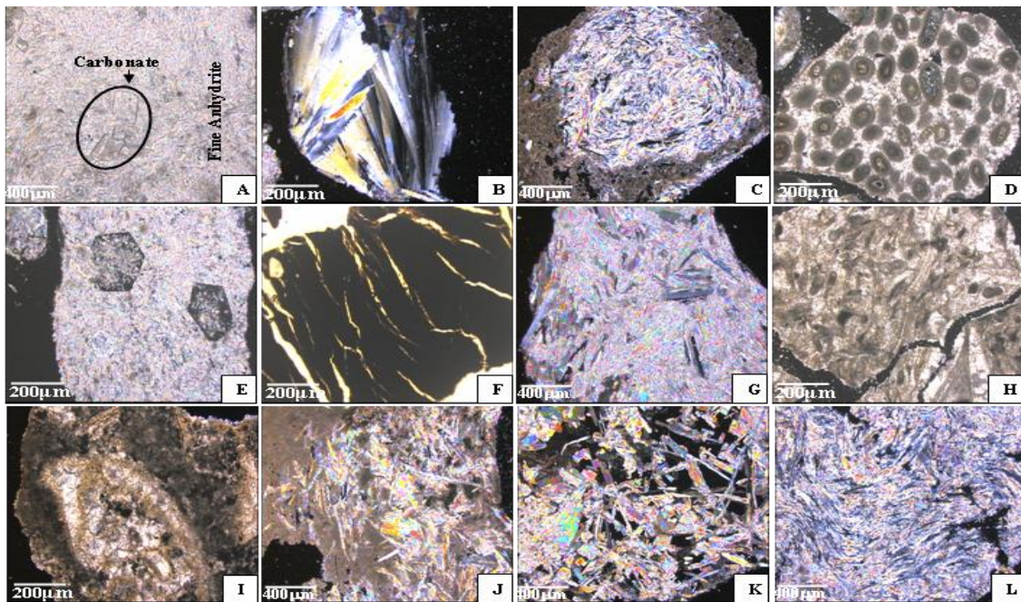
Fig.2- Evaporitic textures observed in the cap rock of Kupal oil field:
