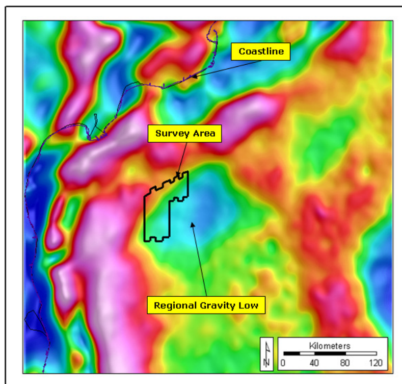
Figure 1. Regional Gravity Data (Sandwell and Smith 2008). 2.2 g/cc Bouguer Correction. Band Pass Filtered 40 – 300 km. Red to blue colors are high to low values. Survey area is at the edge of a regional gravity low.
