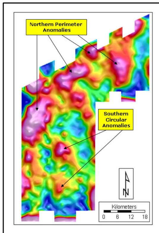
Figure 3. Detailed Gravity Data. 2.2 g/cc Bouguer Correction. High Pass Filtered 20 km. Red to blue colors are high to low values. Map shows the gravity anomalies at the northern perimeter and the southern portion of the survey area.
