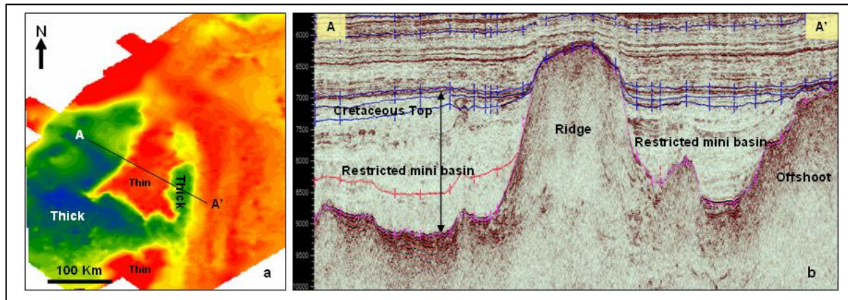
Figure 5 : a) Isopach map between Basement and Cretaceous Top showing varying thickness in the area ( Red – less thick , blue/green - Higher thickness). b) A seismic profile along AA' (marked in figure a) depicting seismic character of the sediments filling the lows.
