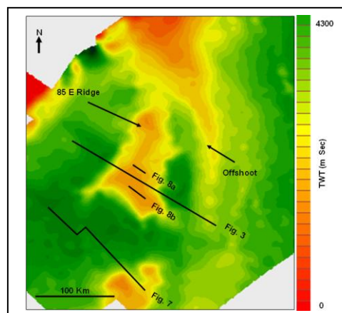
Figure 2: Basement Structure map showing Ridge trend in the area. Locations of various seismic profiles area marked on the map
