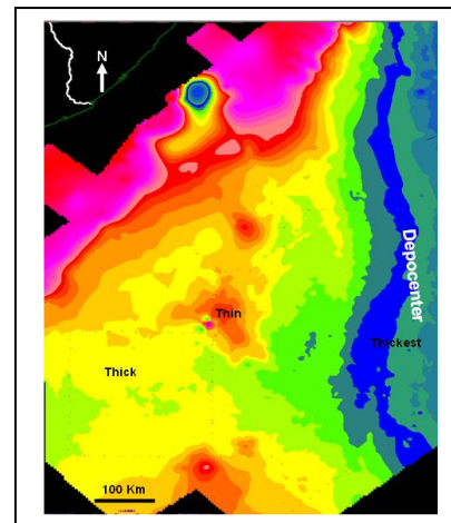
Figure 6: Isopach for Tertiary sediments showing sediment fairway from north. Higher thicker sediments are present towards deeper basinal part in the eastern part of the area. (Red – less thick, blue/green - Higher thickness)
