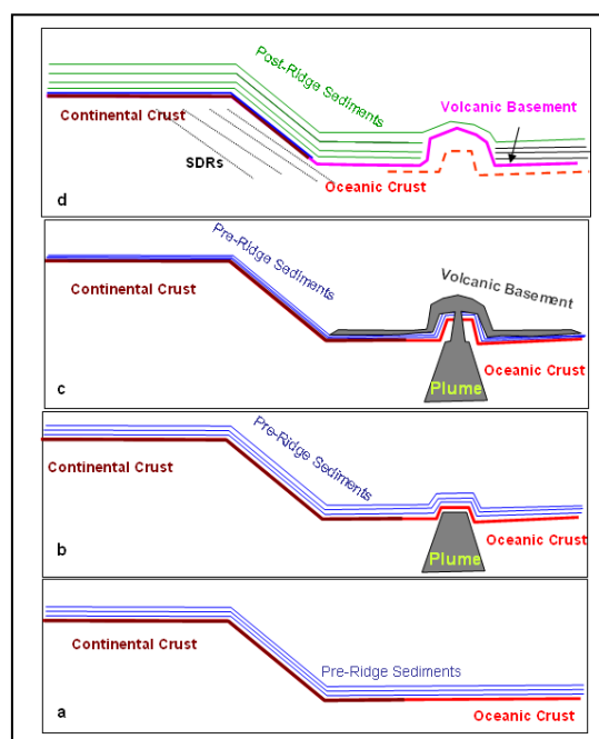
Figure 4: Schematic diagram showing conceptualized model for ridge evolution, and its relation to pre and post ridge sedimentation
