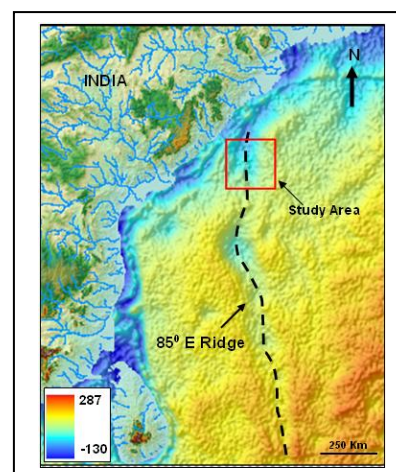
Figure 1: Bouguer gravity map showing gravity low along 85° East Ridge. The study area is shown in the box.
