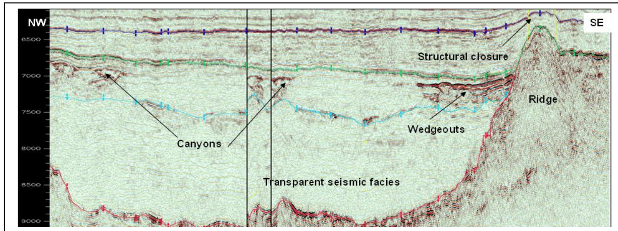
Figure 7: A representative seismic section showing interpreted channelised features in Cretaceous sediments. These are characterized by chaotic seismic reflectors and are seen to be wedging out against basement
