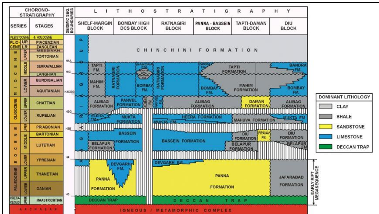
Figure 2 – Generalized Litho-Stratigraphy of Mumbai Offshore Basin.
