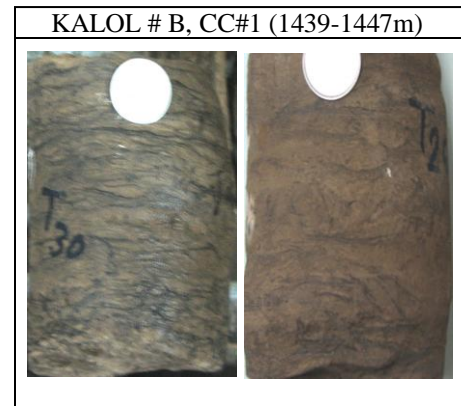
Close up of selected core segments showing burrows and lenticular structures in intertidal sandflat complex
