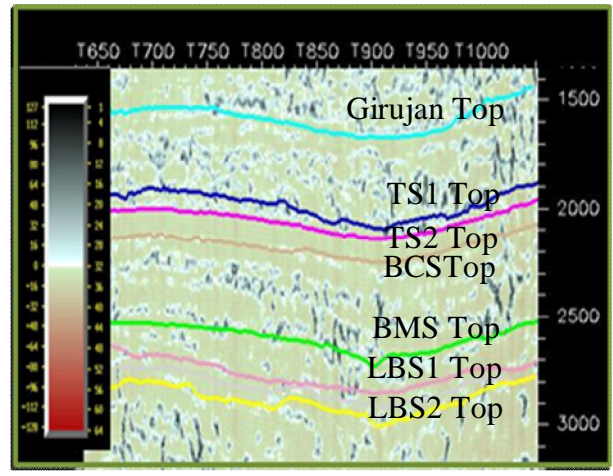
Figure 4. Overlay of Inline 1500, Trace shows data from the new seismic attribute volume and colour from input seismic volume.
