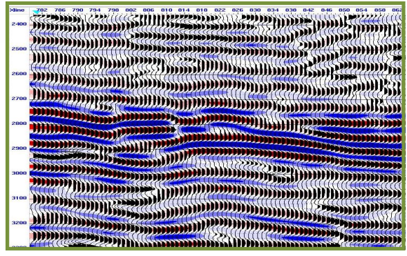
Figure 4. Overlay of Inline 1500, Trace shows data from the new seismic attribute volume and colour from input seismic volume.
