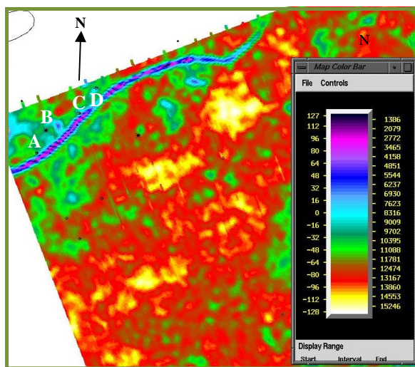
Figure 7. RMS amplitude from the input seismic volume observed between the producing horizons TS1, TS2 and the set of wells A, B, C and D, as shown in dots. The C and D wells fall in different lithology (Sky colour) than the other producing wells A and B (Green colour). Although, it is known that A, B, C and D are producing from the same lithology.
