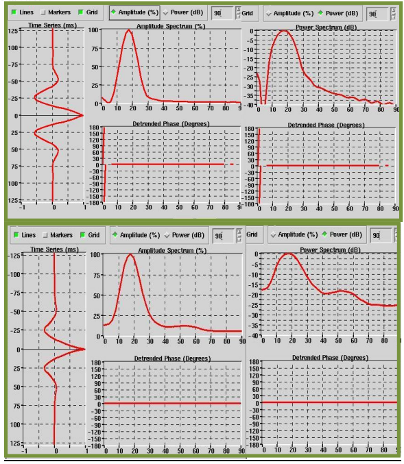
Figure.2. (Above) Spectrum from input Seismic volume. (Below) Spectrum from new seismic attribute volume(Vattr). The latter shows the sharpness of wavelet with reduction of side lobes along with the broadness in power spectrum.
