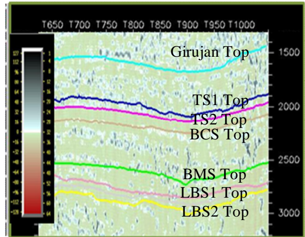
Figure 5. Inline 1500 (Above) From coherency output of input seismic volume.(Below) From coherency output of new seismic attribute volume. The latter shows the smoothing and sharpening of the fault features in time section.
