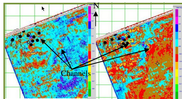
Figure 10. RMS amplitude in windows of 10ms from the P-impedance volume of input seismic (left) and Vatttr volume (right). All the producing wells, black dots, are placed over the channel sandbody (right) which is not the case with input seismic (left). It confirms the observed results at the set of wells.
