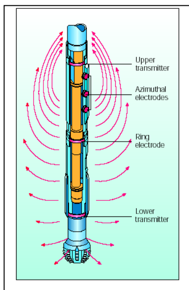
Figure 1: The LWD laterolog resistivity tool.
