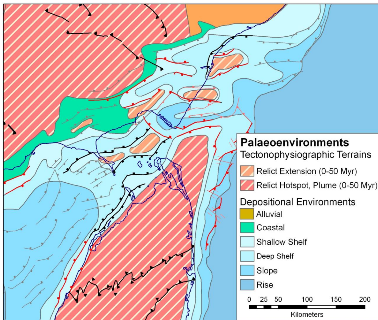
Figure 2: Campanian (79Ma) palaeogeographic map of the Cauvery and northern Mannar Basin, showing the relationship between the tectonophysiographic terrains (source areas) and depositional areas (sink areas). Small highs within the southern Cauvery Basin are considered sedimentary sources for locally derived turbidites which form potential reservoirs.
