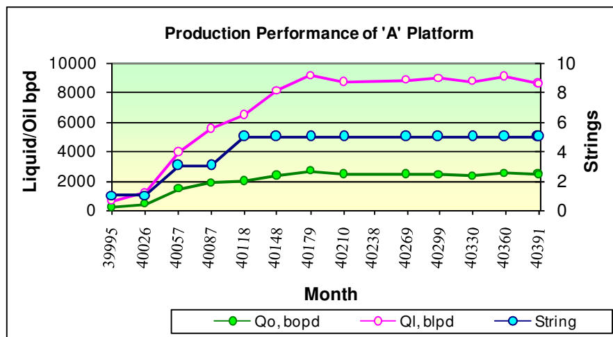
Fig 10: Production Performance of Platform 'A'
