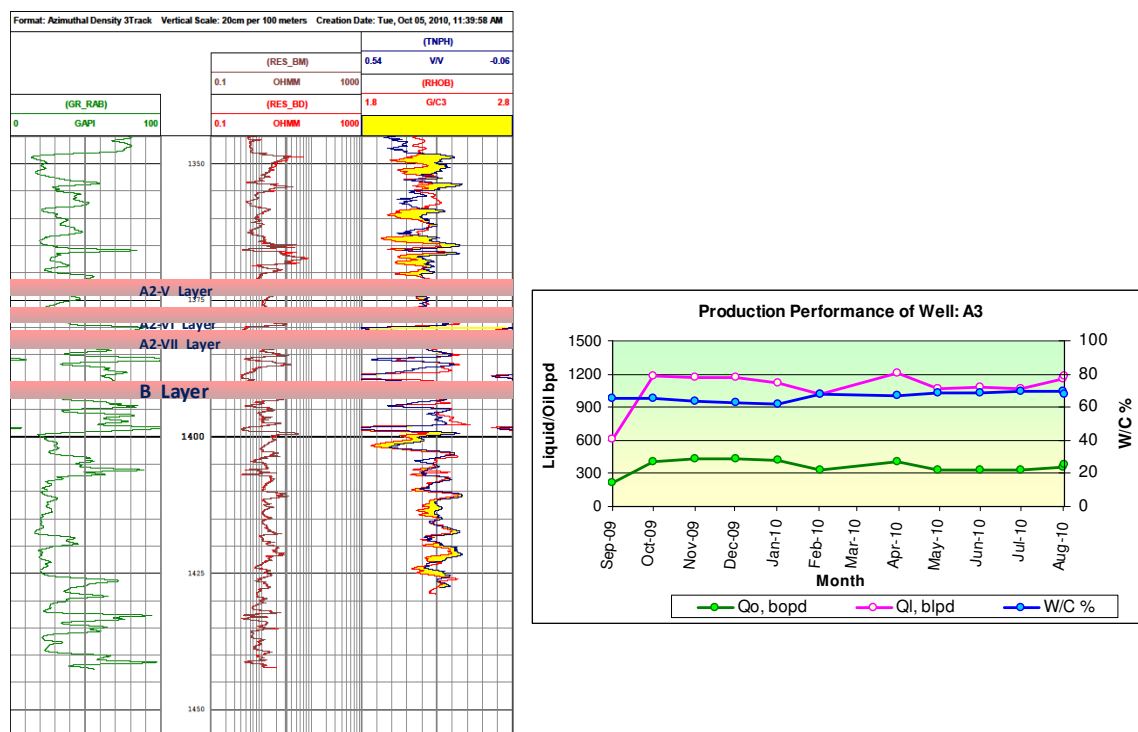
Fig 7: Well logs & Production Performance of Well 'A3'
