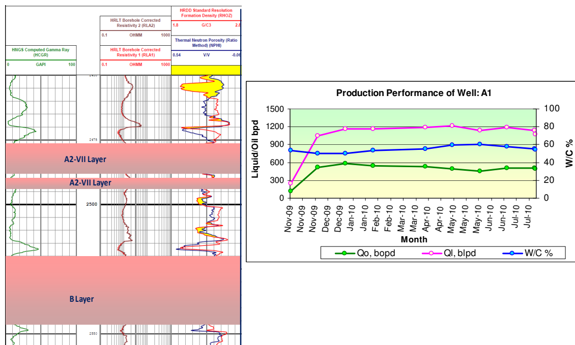
Fig 5: Well logs & Production Performance of Well 'A1'
