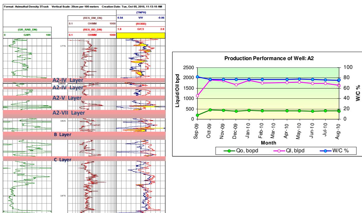
Fig 6: Well logs & Production Performance of Well ‘A2’
