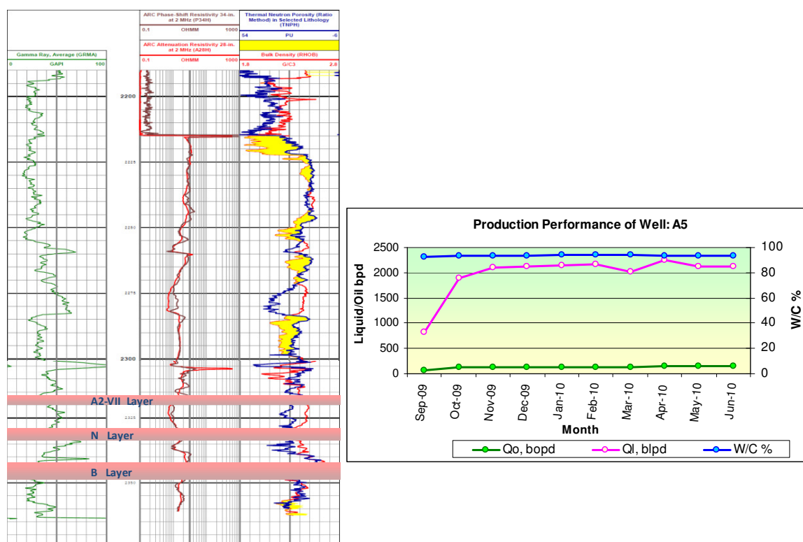
Fig 9: Well logs & Production Performance of Well 'A5'
