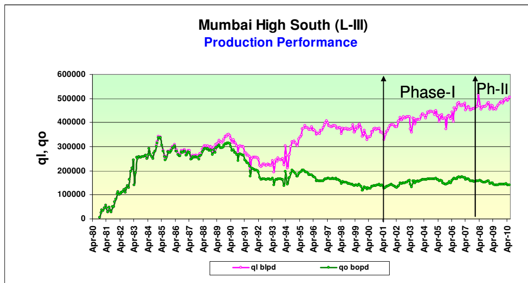
Fig 2: Production Performance of Mumbai High South
