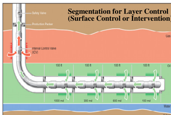
Fig. 11 Segmented completion
