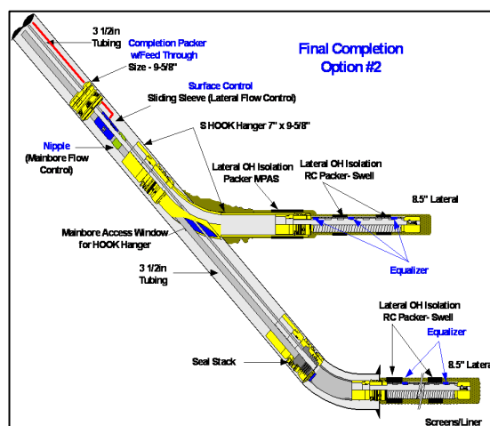
Fig. 10 Level- 3 completion in a Typical Well
