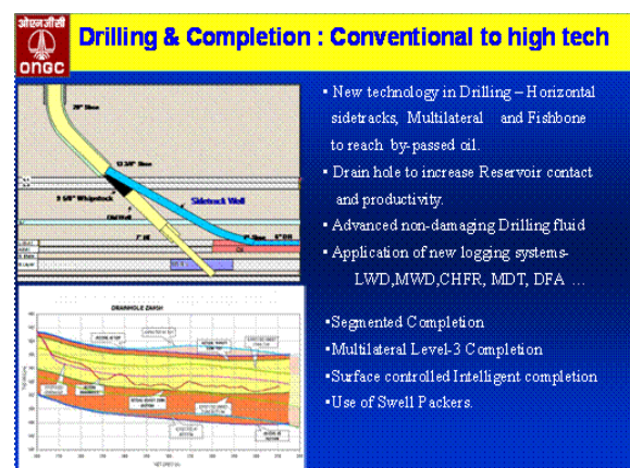
Fig.3 Drilling & Completion
